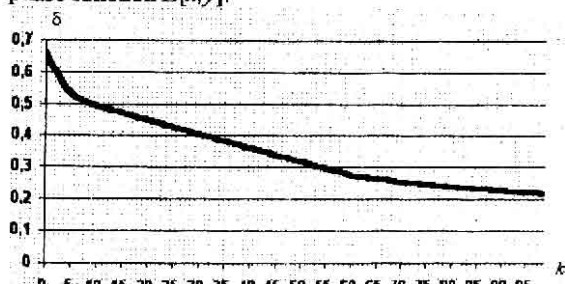
Fig. 4. R.m.s. error of reconstruction \delta vs the number of iterations
