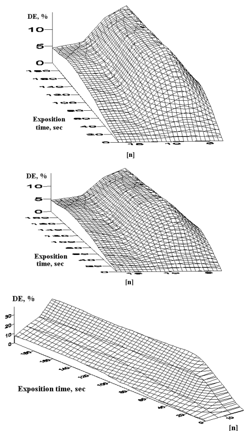
Fig. 2. The diffraction efficiency vs the time of exposure by the light of 10 \text{ mW/cm}^2 for the SD DG layers with the gelatin concentrations: a - 3 %, b- 7 %, c- 10 %. [n] = glycerol concentration
